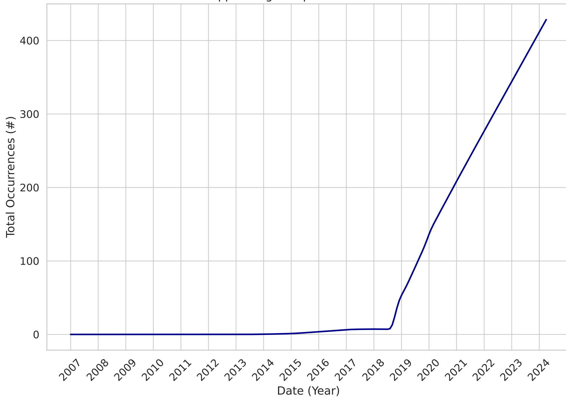
Suppressing Exception Context Trend
